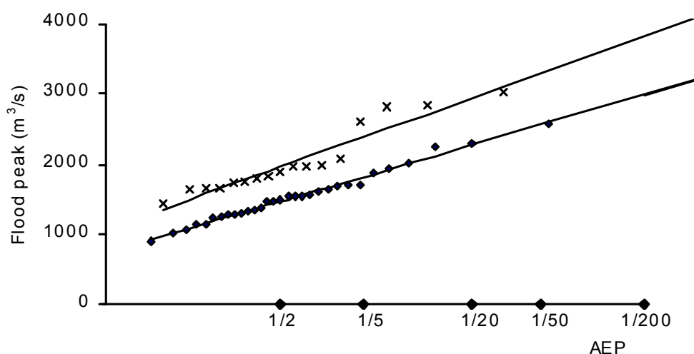
Figure 3.8: Flood frequency analysis for the Lake Te Anau 3-day annual maxima for 1947–1977 (lower line) and 1978–1994 (upper line).
