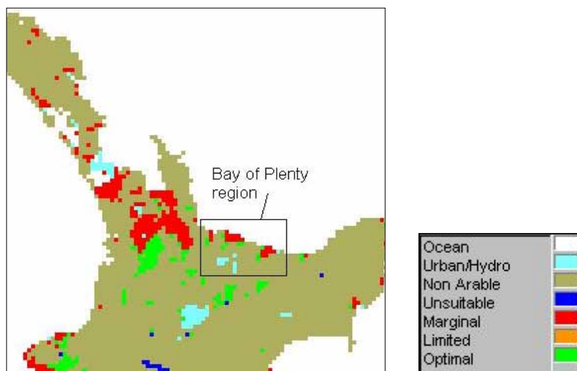
Figure 5.1: An example of a screening assessment of kiwifruit suitability, using a mid-range climate scenario for the year 2095.
