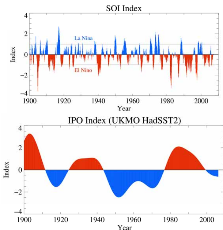
Figure 3.4: Time series of Southern Oscillation Index (SOI, upper panel) and Interdecadal Pacific Oscillation (IPO, lower panel) from 1900.
