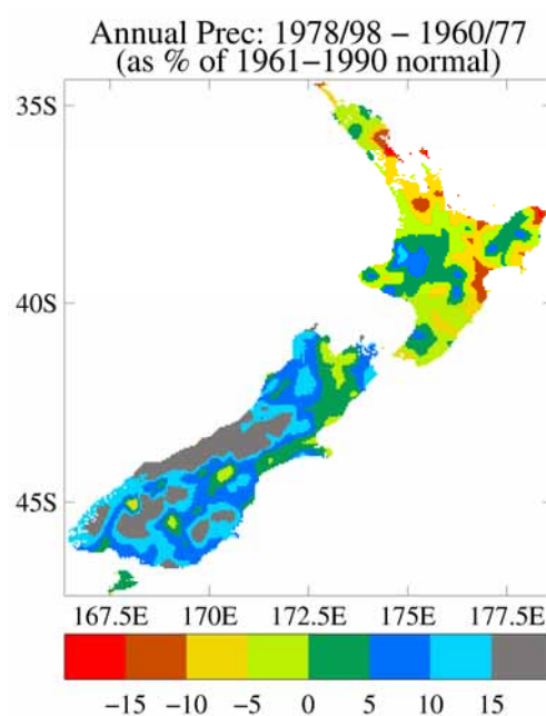
Figure 3.5: Percentage change in average annual rainfall for 1978–1998 compared to 1960–1977.
