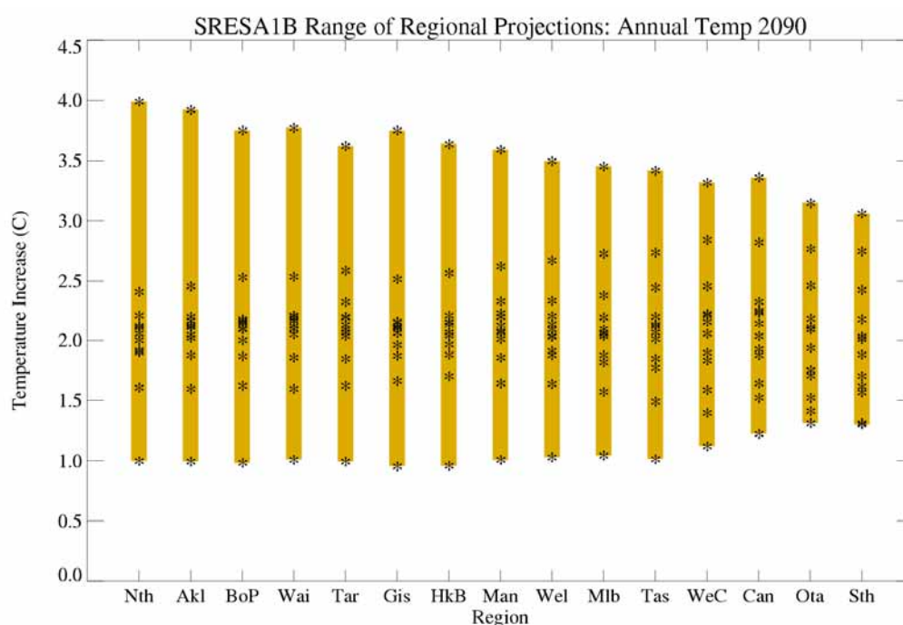
Figure A3.7: Range in projected annual temperature change (in °C) by 2090 for the A1B emissions scenario.
