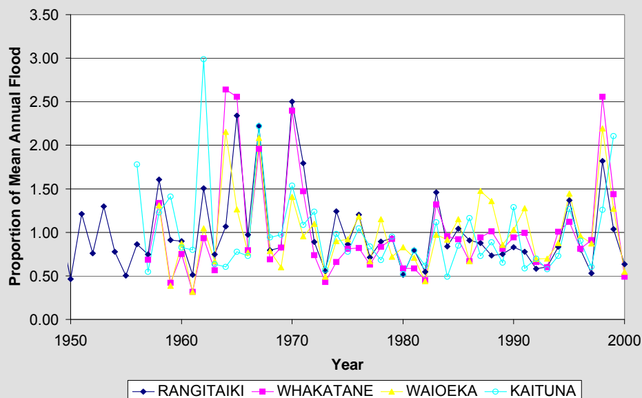
Figure Box 4.1: Annual maximum flow as a proportion of the mean annual flood for the Rangitaiki, Whakatane, Waioeka and Kaituna rivers in the Bay of Plenty 1950–2000.
